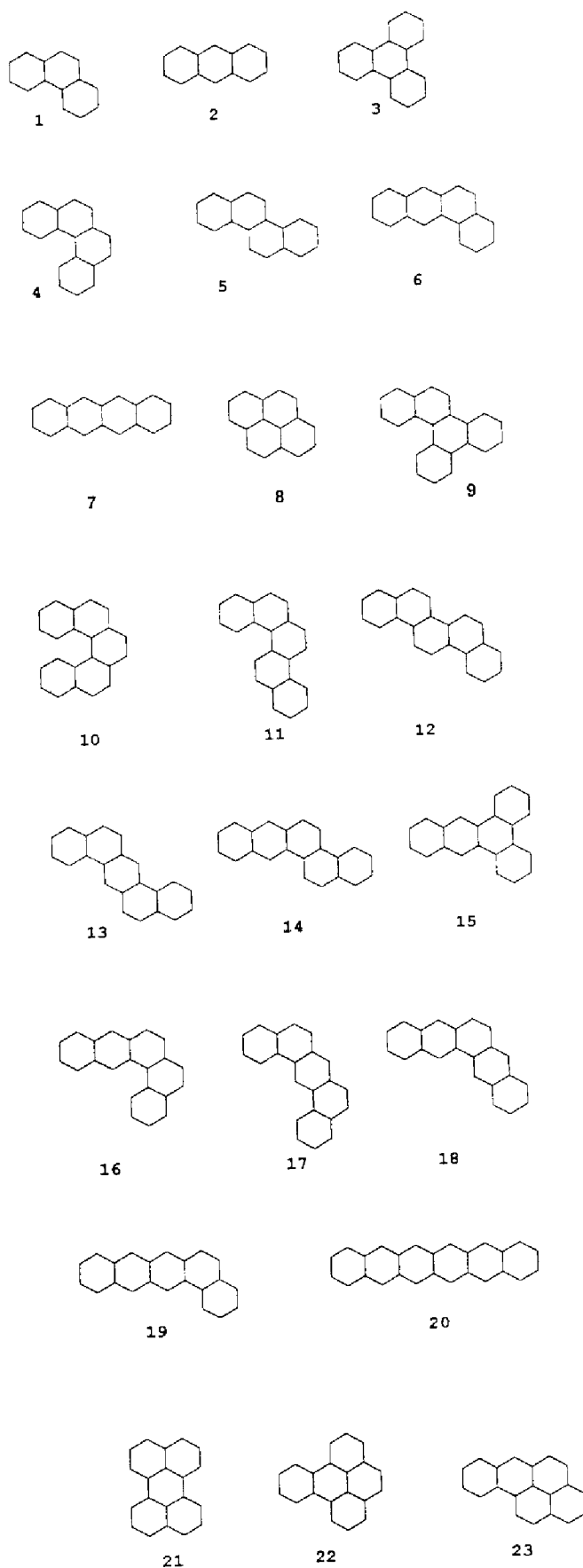
Figure 1. Polyhexes with 3, 4 and 5 benzenoid rings whose distance ID numbers MINID and MINSID are presented in Table II.
